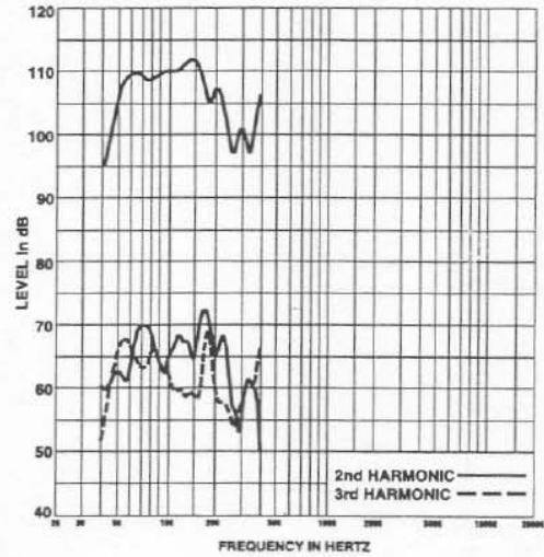
FIGURE 6 — Harmonic Distortion
